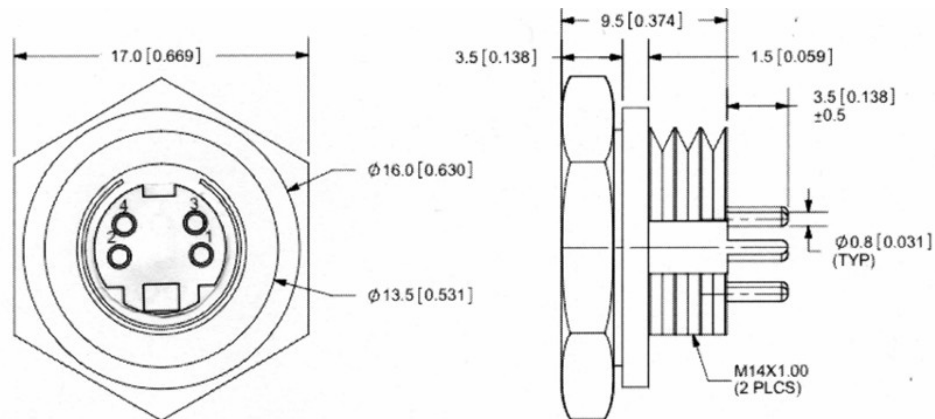
Figure 2.2.1.1 - Mini DIN-4 pin RV-C Service Port Connector
