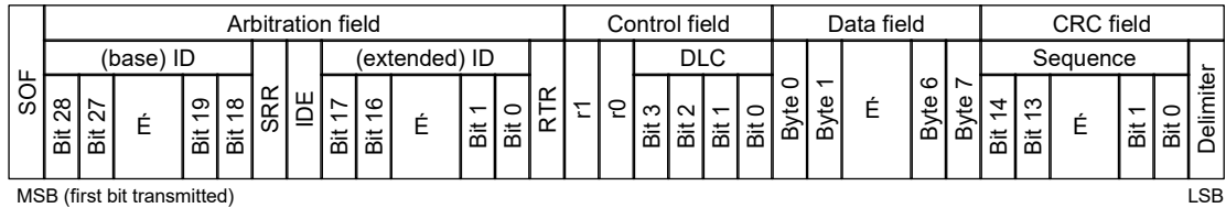
Figure 3.1 CAN data frame structure
