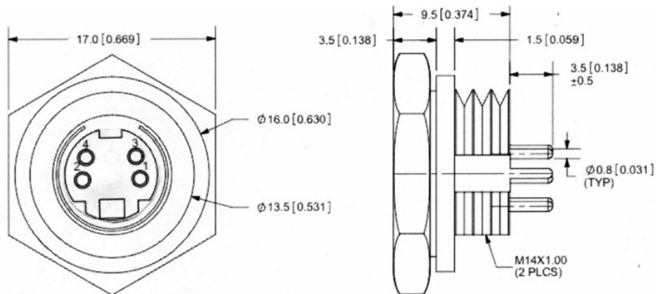
Figure 2.2.1.1 - Mini DIN-4 pin RV-C Service Port Connector
