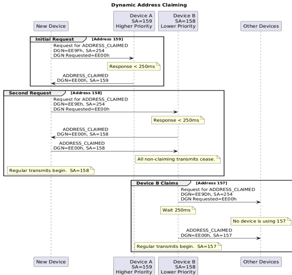
Figure 3.3.2.3 – Dynamic Addressing Sequence
